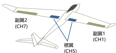
2AIL+1FLP (AF1)
